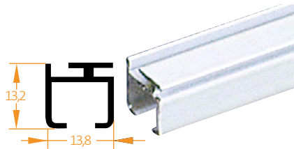
Riel barras (6mts.)*
